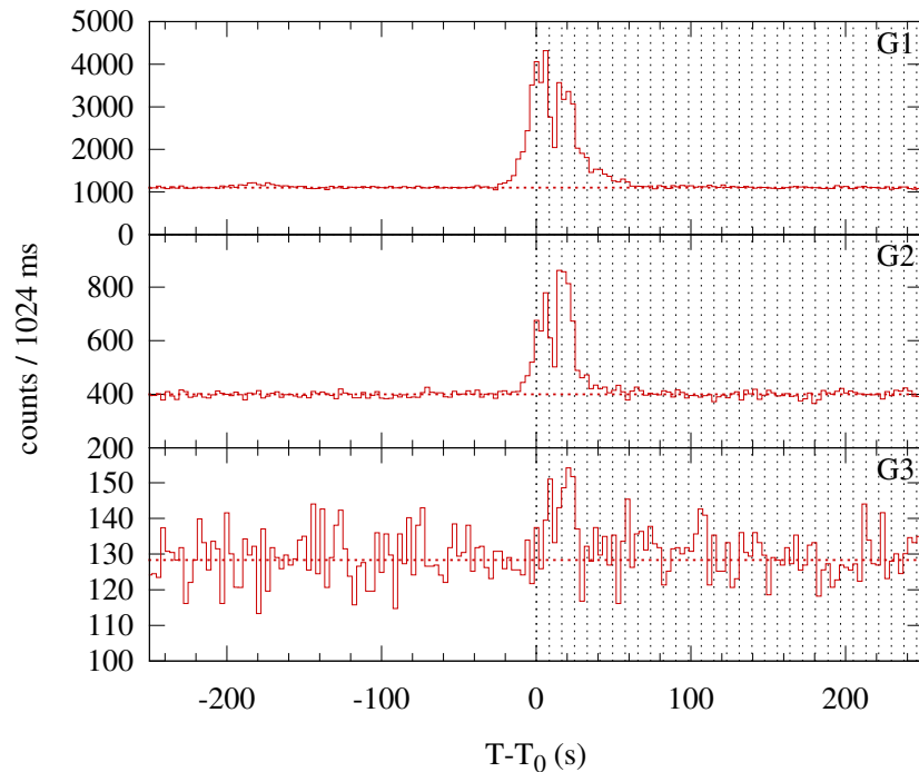
Konus-WIND S2 SOL2004-07-17T19:17 (C5.3) T 0 = 69428.586 s UT (19:17:08.586)
