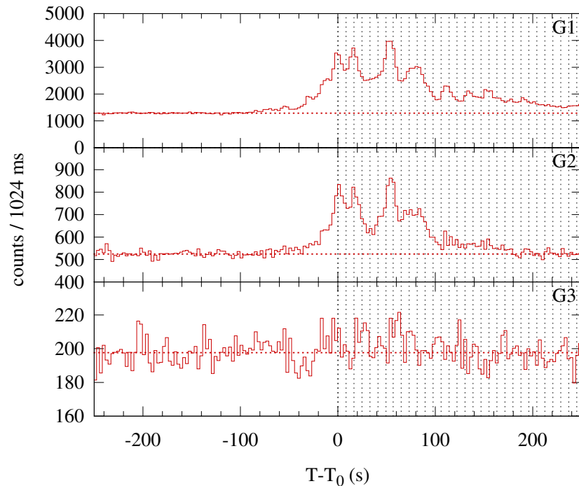
Konus-WIND S2 SOL2005-08-03T04:58 (M3.4) T_0 = 17907.794 s UT (04:58:27.794)
