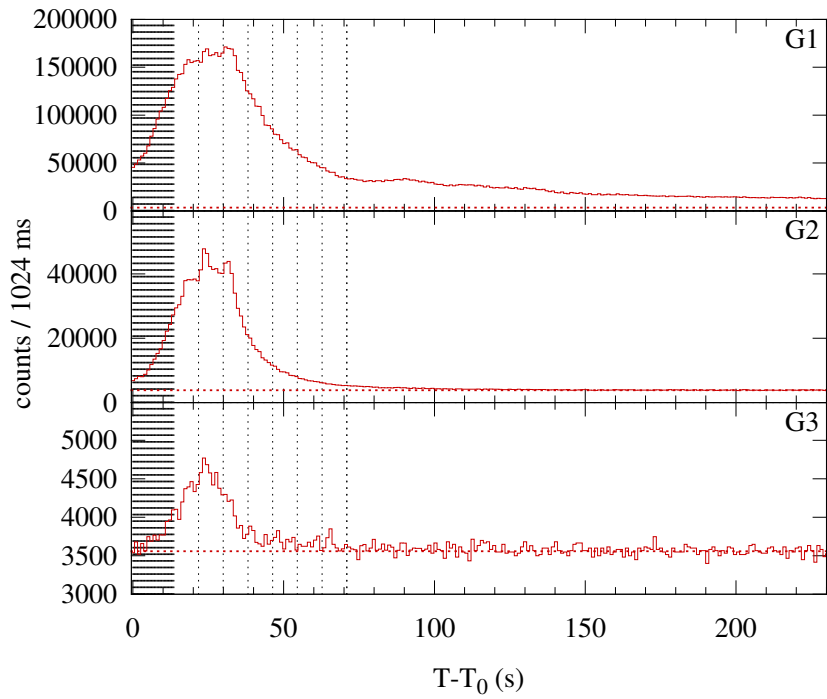
Konus-WIND S2 SOL2005-09-13T19:22 (X1.5) T_0 = 69772.711 s UT (19:22:52.711)
