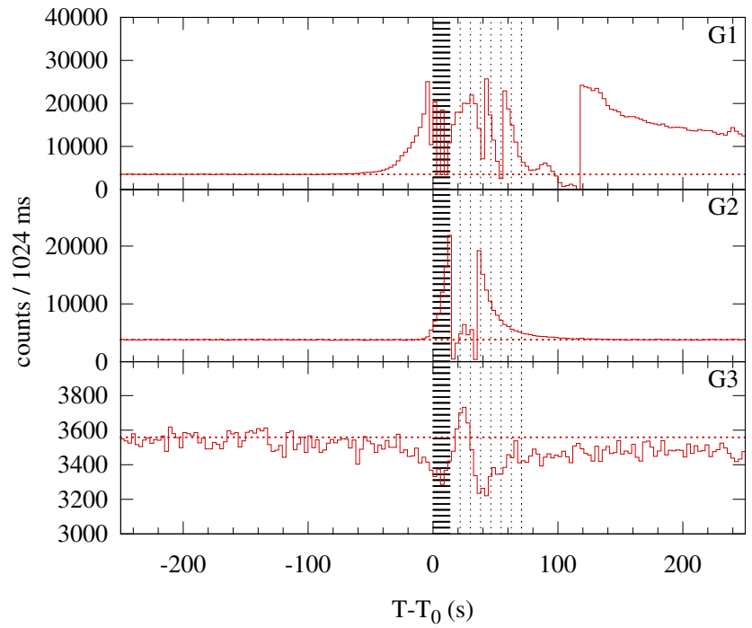
Konus-WIND S2 SOL2005-09-13T19:22 (X1.5) T_0 = 69772.711 s UT (19:22:52.711)
