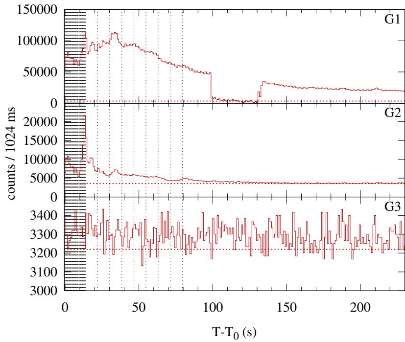
Konus-WIND S2 SOL2005-09-13T23:19 (X1.7) T_0 = 83980.362 s UT (23:19:40.362)
