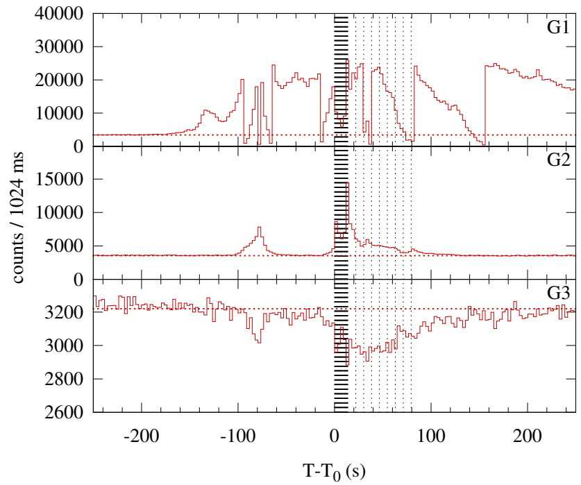
Konus-WIND S2 SOL2005-09-13T23:19 (X1.7) T_0 = 83980.362 s UT (23:19:40.362)
