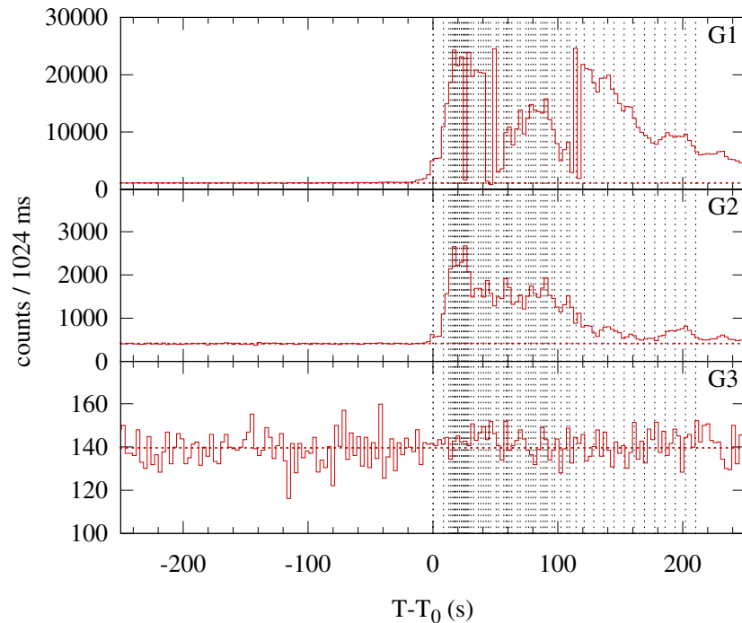
Konus-WIND S2 SOL2005-12-02T10:09 (M7.8) T 0 = 36581.866 s UT (10:09:41.866)
