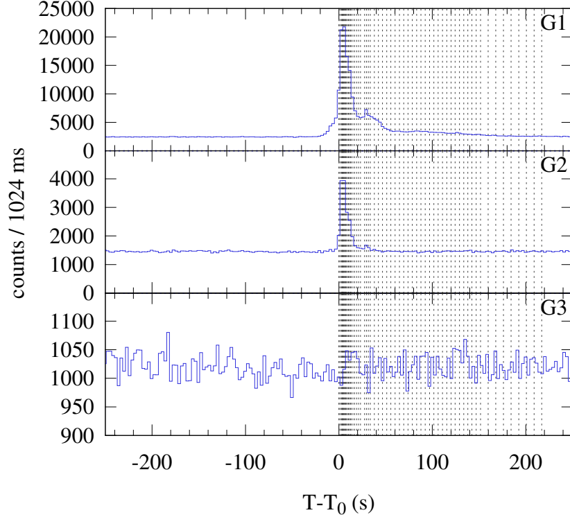
Konus-WIND S2 SOL2024-05-12T00:42 (M3.2) T 0 = 2538.33 s UT (00:42:18.33)
