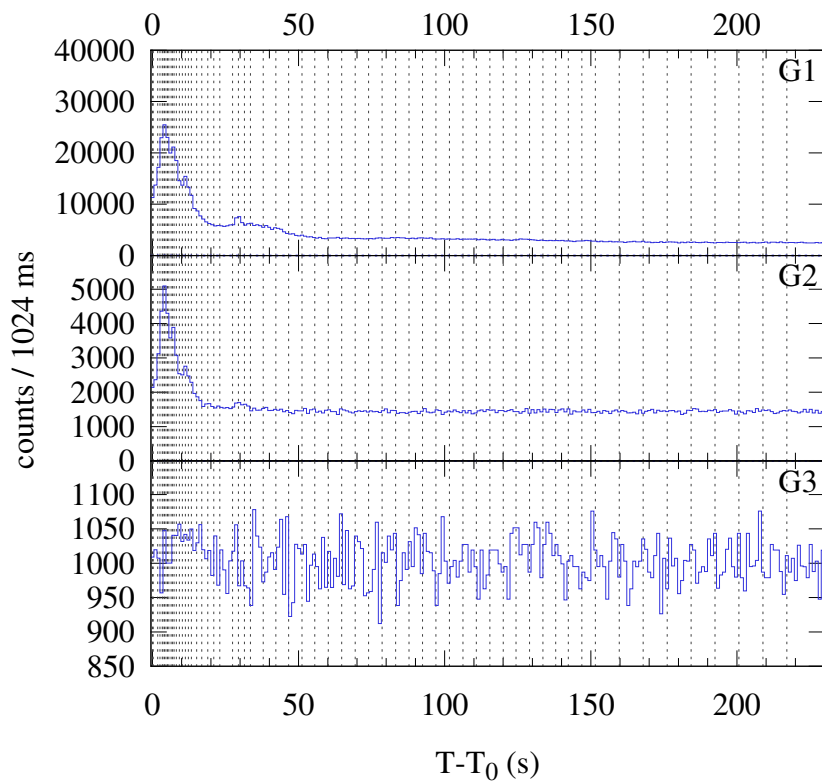
Konus-WIND S2 SOL2024-05-12T00:42 (M3.2) T 0 = 2538.33 s UT (00:42:18.33)
