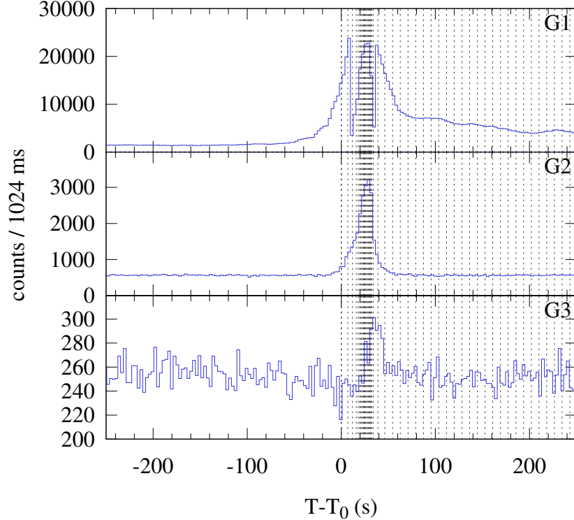
Konus-WIND S2 SOL2024-05-12T16:18 (X1.0) T_0 = 58733.610 s UT (16:18:53.610)
