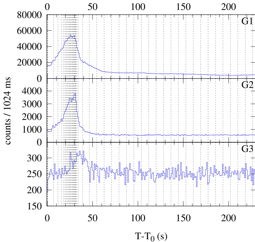
Konus-WIND S2 SOL2024-05-12T16:18 (X1.0) T_0 = 58733.610 s UT (16:18:53.610)
