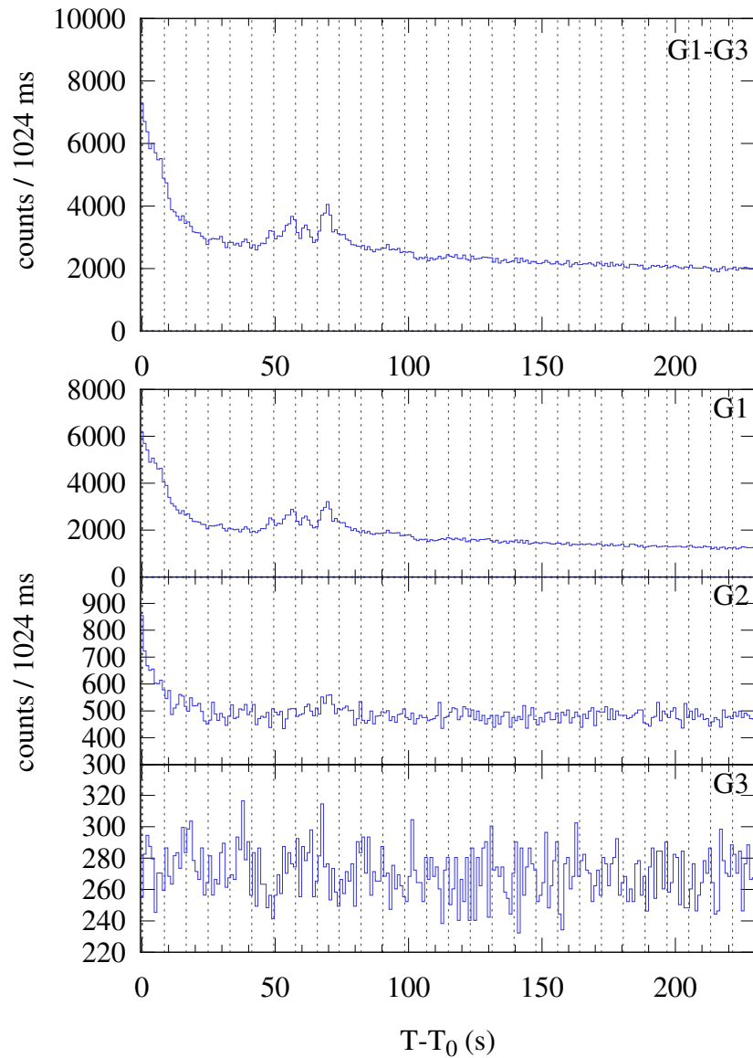
Konus-WIND S2 SOL2024-05-23T02:13 (M4.2) T_0 = 8032.110 s UT (02:13:52.110)
