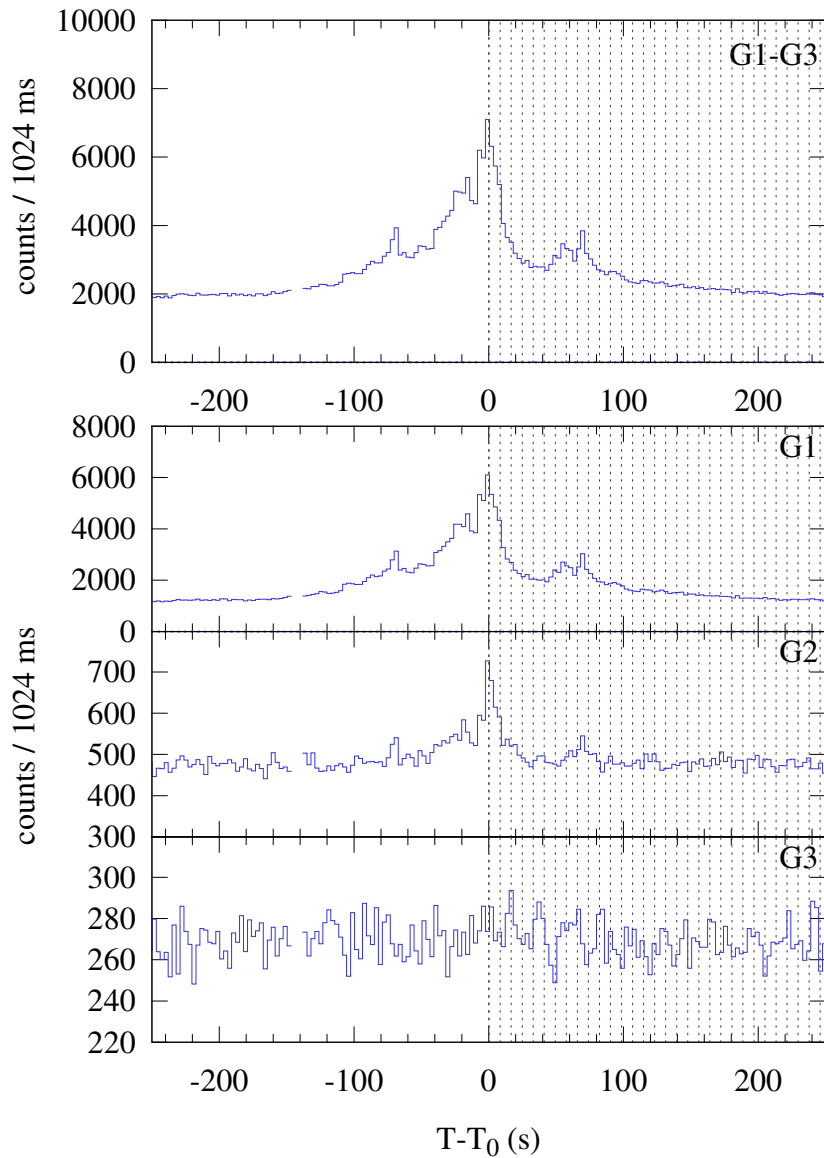
Konus-WIND S2 SOL2024-05-23T02:13 (M4.2) T_0 = 8032.110 s UT (02:13:52.110)
