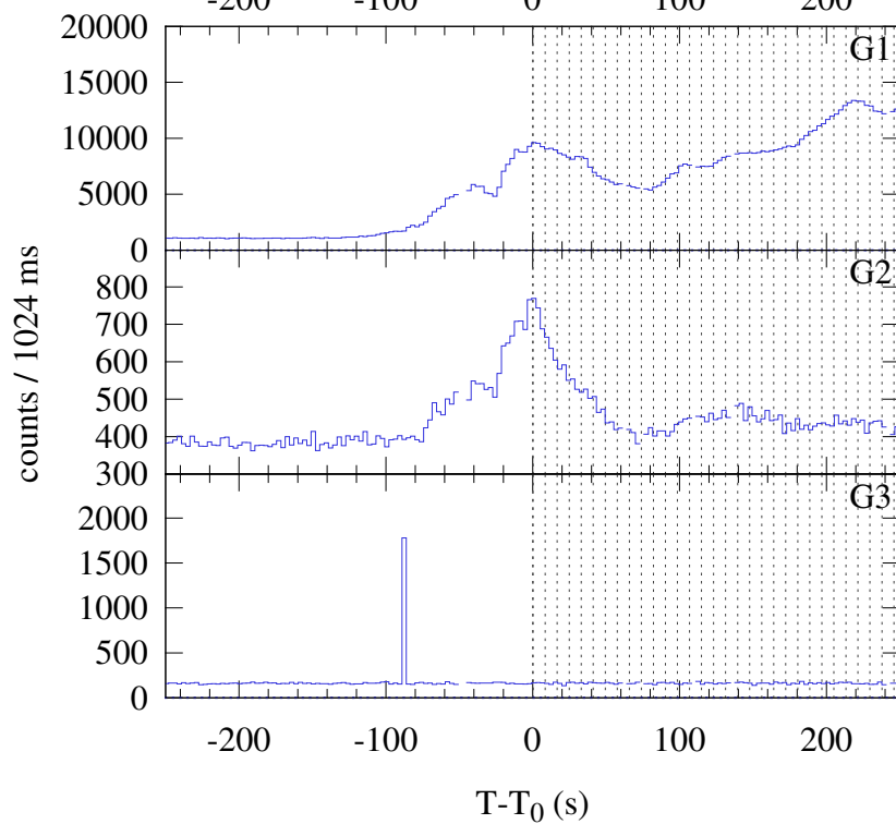
Konus-WIND S2 SOL2024-05-27T06:57 (X2.8) T_0 = 25063.470 s UT (06:57:43.470)
