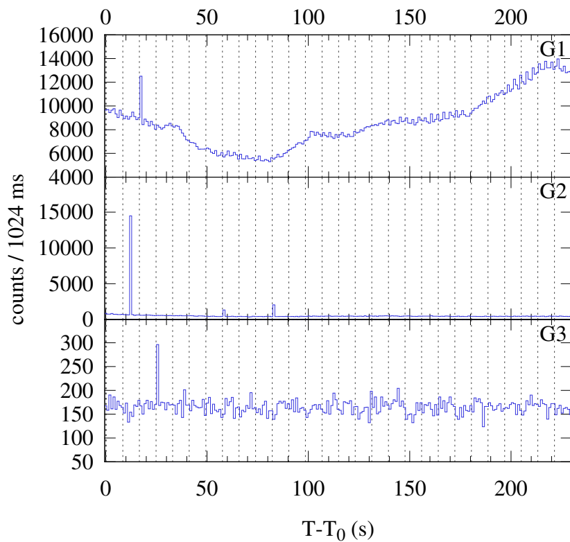
Konus-WIND S2 SOL2024-05-27T06:57 (X2.8) T_0 = 25063.470 s UT (06:57:43.470)
