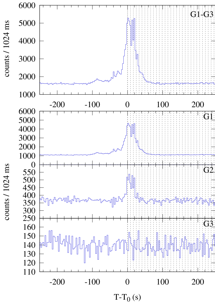
Konus-WIND S2 SOL2024-05-29T18:27 (M2.7) T_0 = 66464.841 s UT (18:27:44.841)
