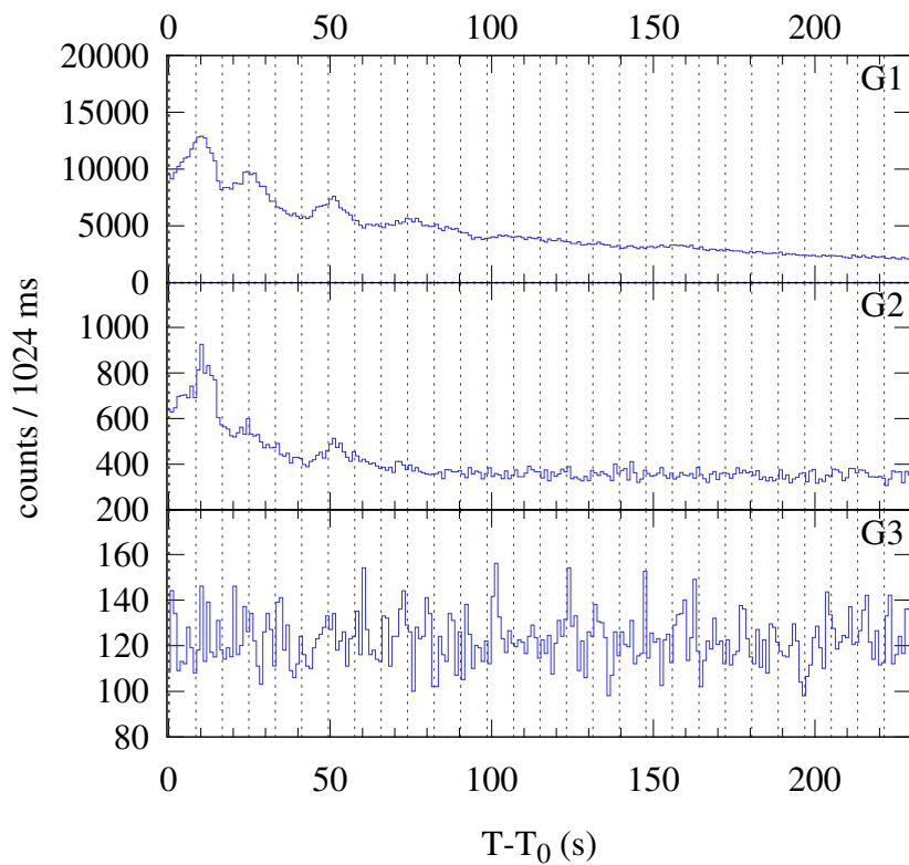
Konus-WIND S2 SOL2024-06-01T18:32 (X1.0) T_0 = 66756.212 s UT (18:32:36.212)
