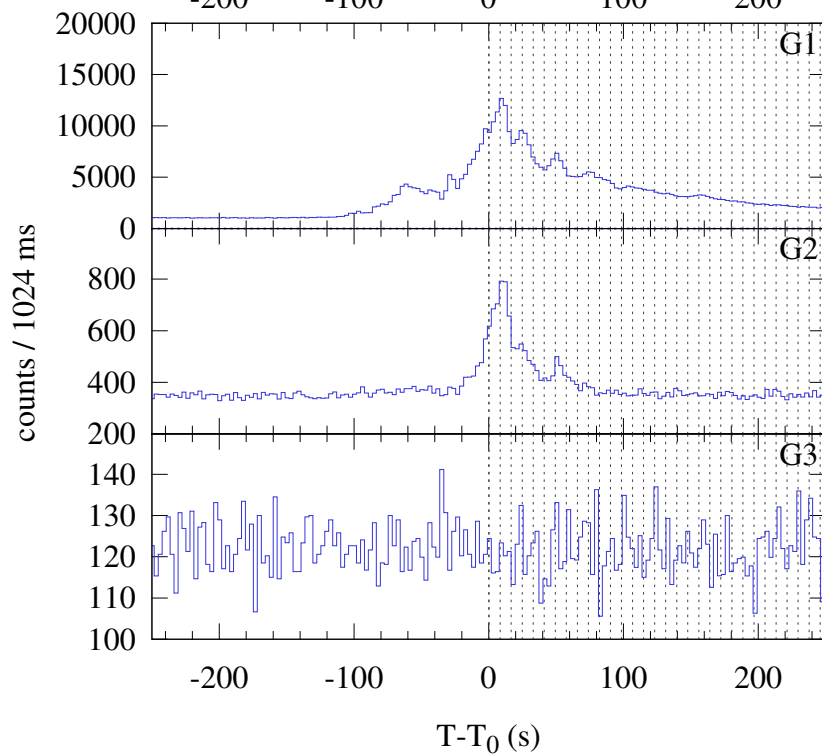
Konus-WIND S2 SOL2024-06-01T18:32 (X1.0) T_0 = 66756.212 s UT (18:32:36.212)
