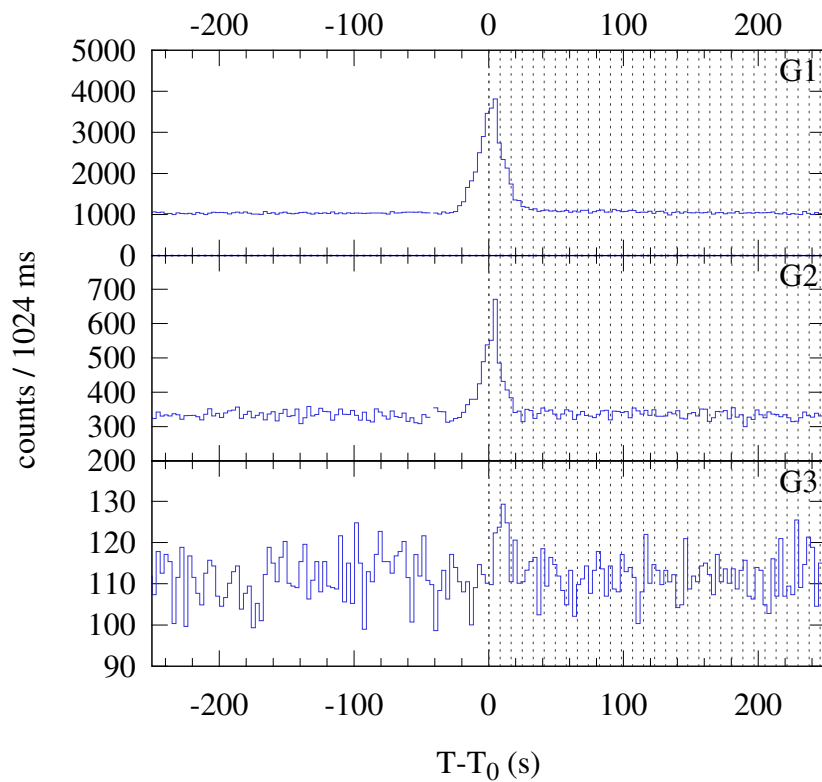
Konus-WIND S2 SOL2024-08-19T09:35 (M1.3) T_0 = 34535.670 s UT (09:35:35.670)
