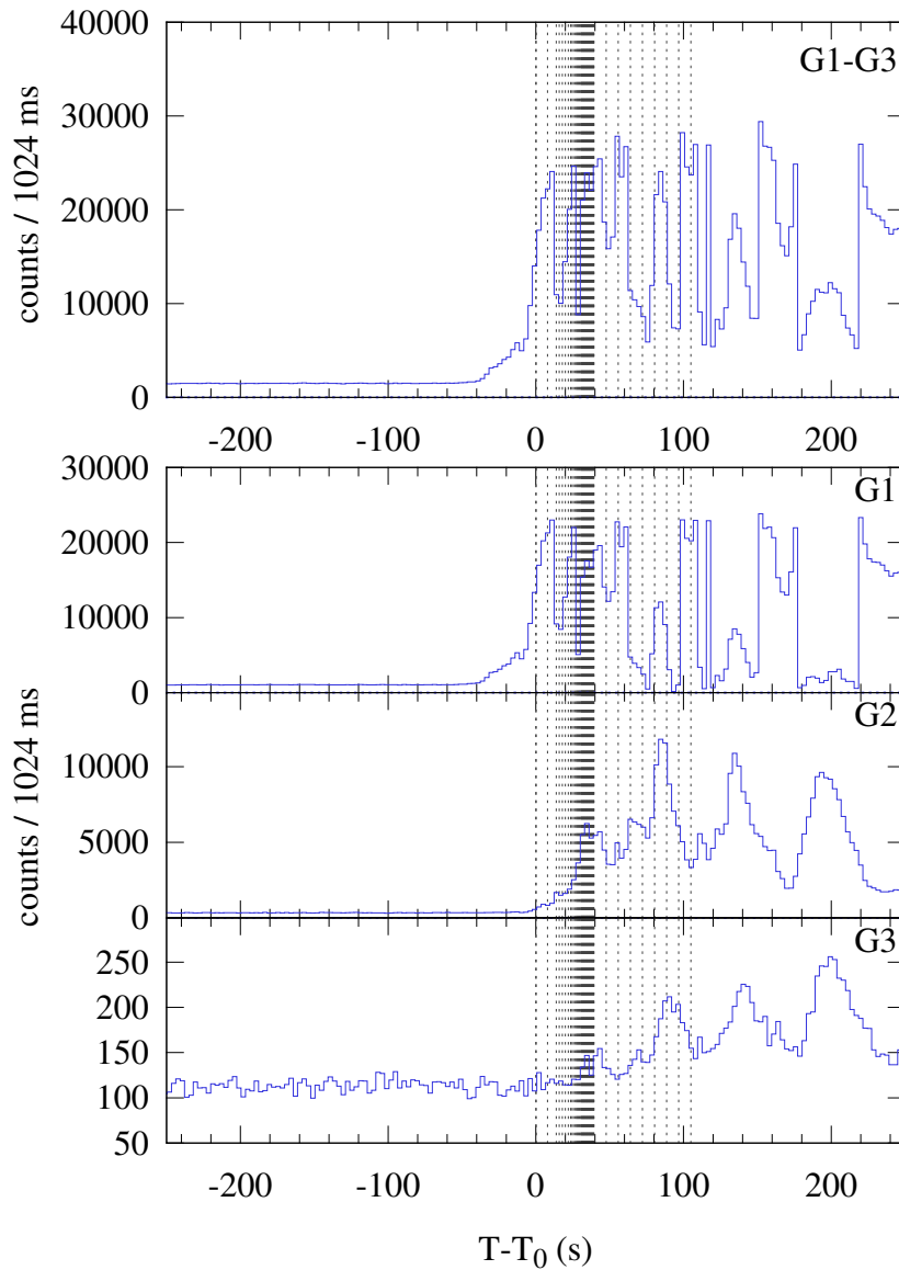
Konus-WIND S2 SOL2024-10-03T12:14 (X9.0) T_0 = 44046.609 s UT (12:14:06.609)
