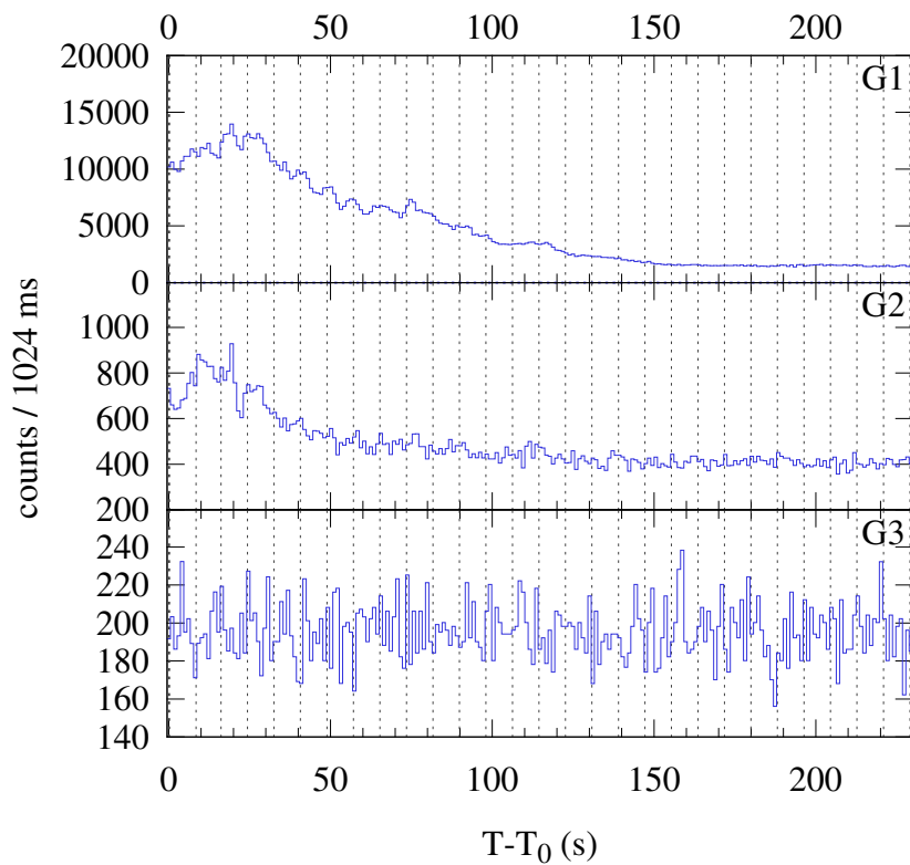
Konus-WIND S2 SOL2024-10-14T00:11 (M3.4) T_0 = 665.337 s UT (00:11:05.337)
