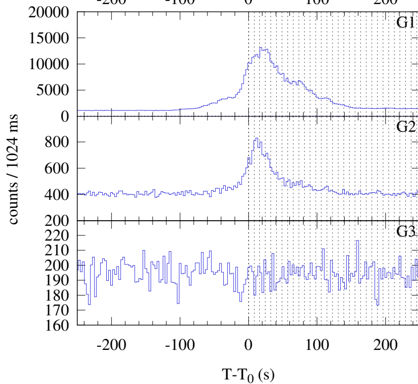
Konus-WIND S2 SOL2024-10-14T00:11 (M3.4) T_0 = 665.337 s UT (00:11:05.337)
