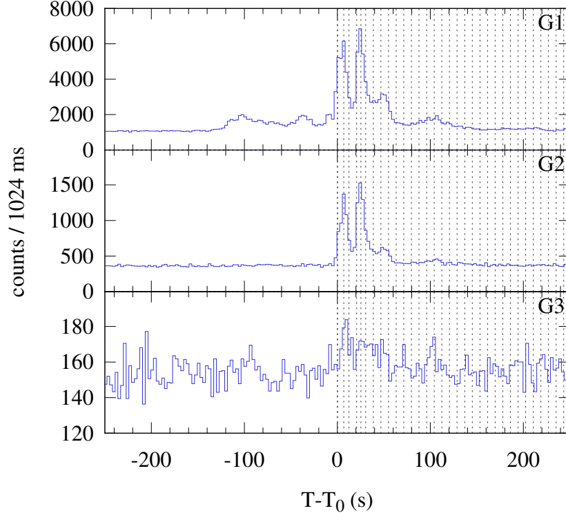
Konus-WIND S2 SOL2024-10-15T18:30 (M2.1) T_0 = 66631.33 s UT (18:30:31.33)
