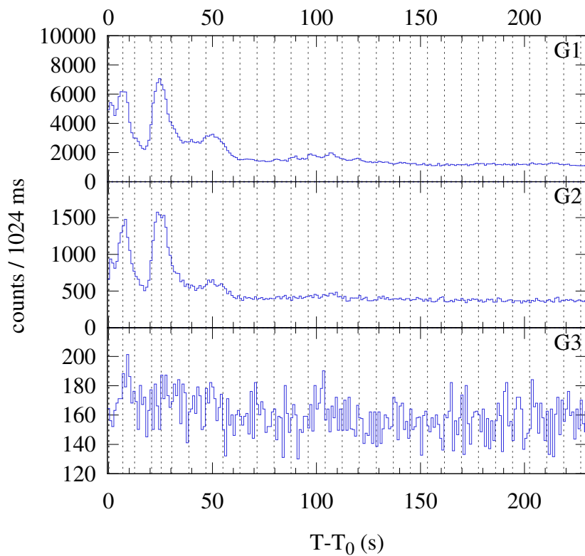
Konus-WIND S2 SOL2024-10-15T18:30 (M2.1) T_0 = 66631.33 s UT (18:30:31.33)
