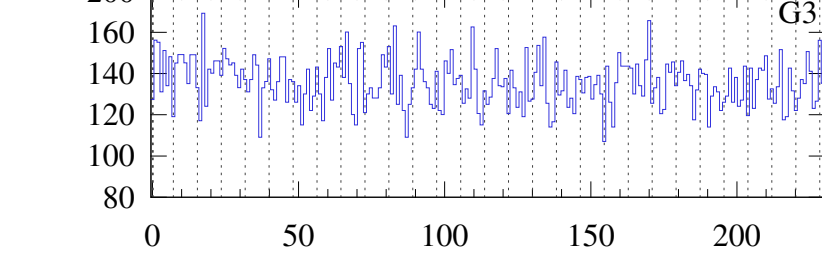
Konus-WIND S2 SOL2024-10-17T05:01 (M2.4) T_0 = 18077.224 s UT (05:01:17.224)
