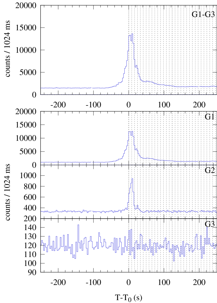
Konus-WIND S2 SOL2024-10-18T23:26 (M4.7) T_0 = 84409.463 s UT (23:26:49.463)
