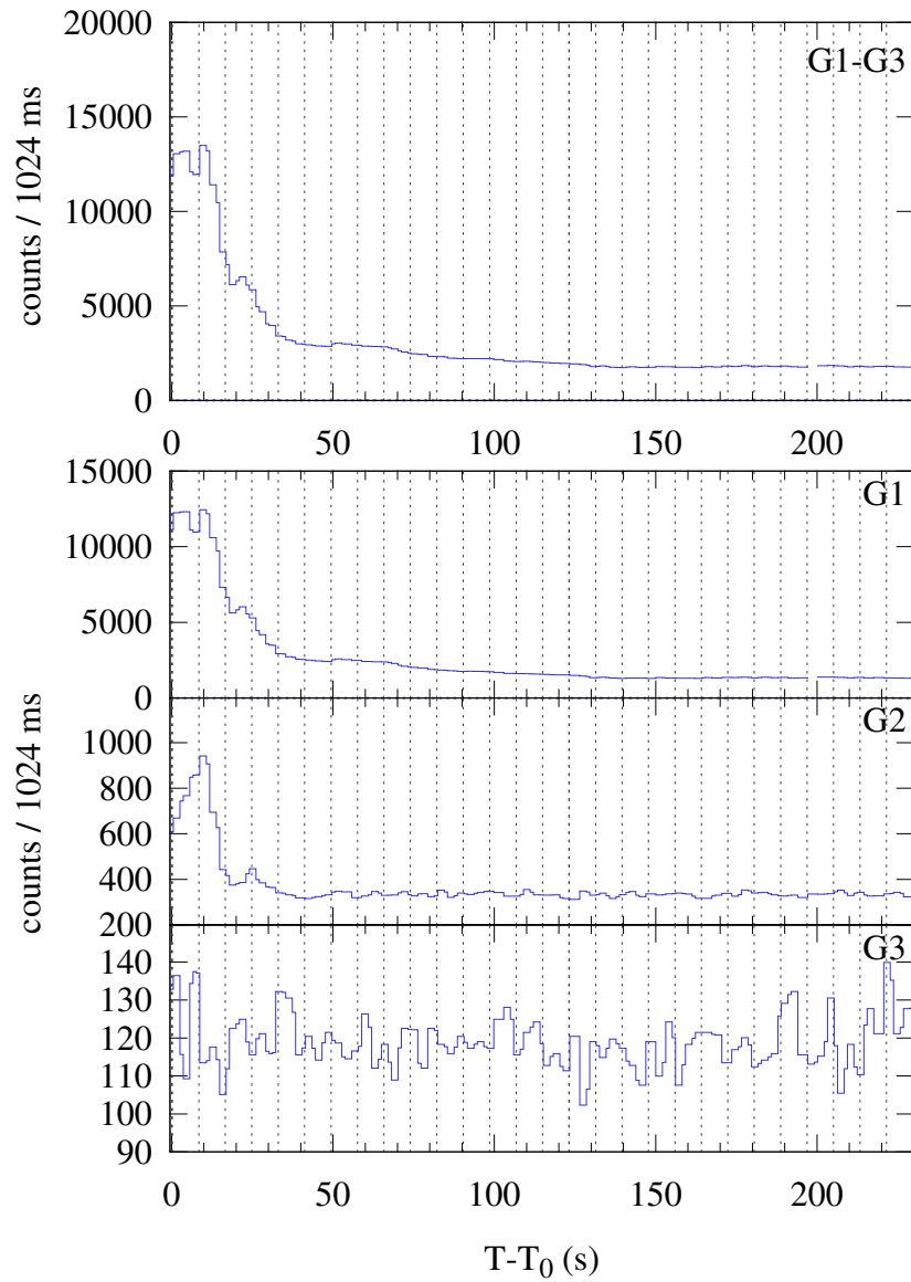
Konus-WIND S2 SOL2024-10-18T23:26 (M4.7) T_0 = 84409.463 s UT (23:26:49.463)
