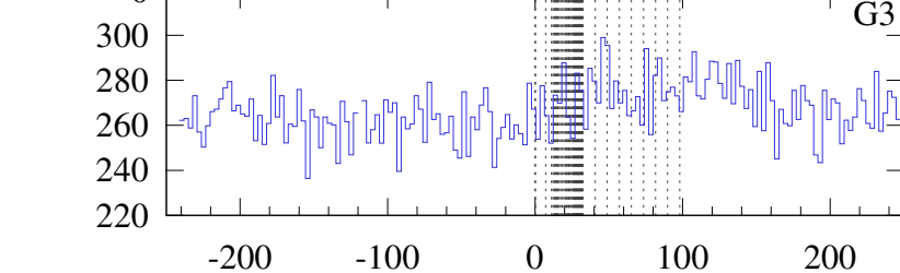
Konus-WIND S2 SOL2024-10-31T21:15 (X2.0) T_0 = 76519.603 s UT (21:15:19.603)
