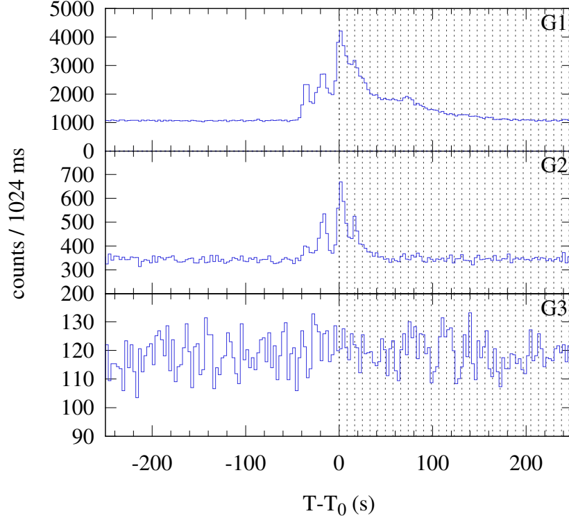
Konus-WIND S2 SOL2024-11-06T08:48 (M5.8) T_0 = 31732.777 s UT (08:48:52.777)
