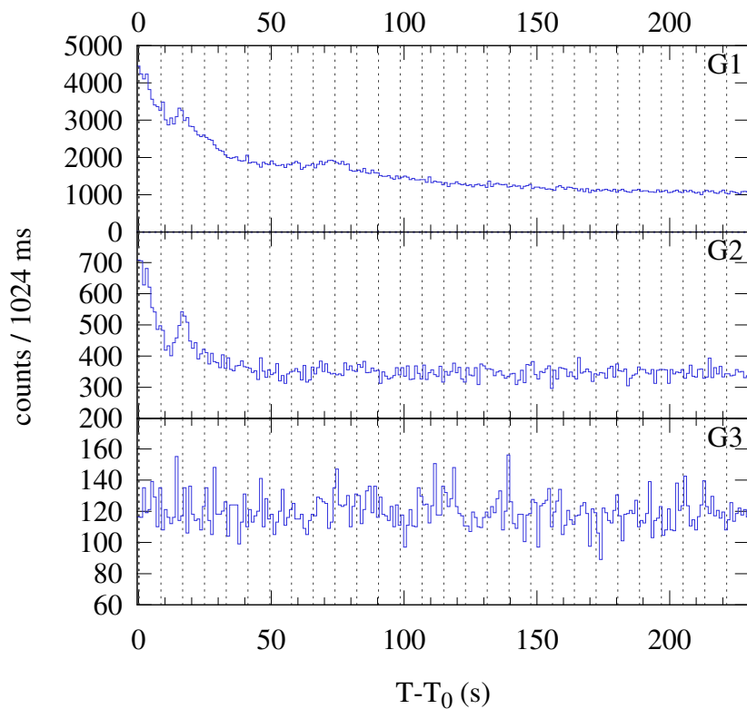
Konus-WIND S2 SOL2024-11-06T08:48 (M5.8) T_0 = 31732.777 s UT (08:48:52.777)
