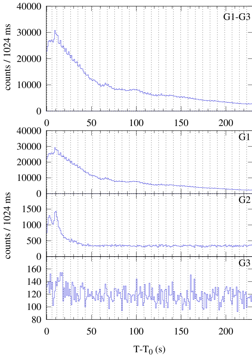
Konus-WIND S2 SOL2024-11-06T13:39 (X2.3) T_0 = 49185.138 s UT (13:39:45.138)
