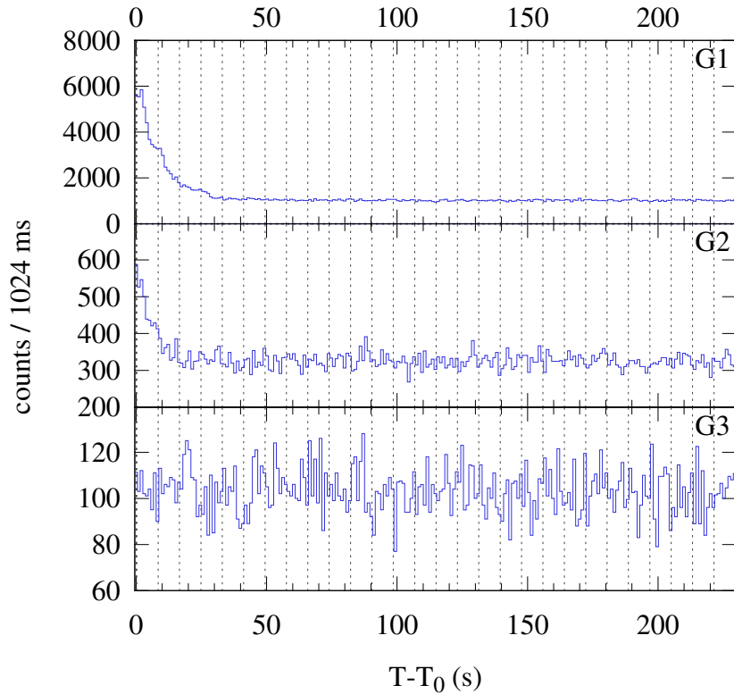
Konus-WIND S2 SOL2024-12-11T11:40 (C5.7) T_0 = 42047.161 s UT (11:40:47.161)
