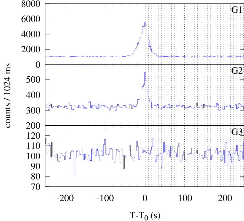
Konus-WIND S2 SOL2024-12-11T11:40 (C5.7) T_0 = 42047.161 s UT (11:40:47.161)
