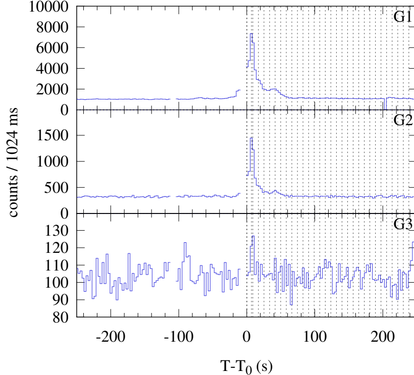
Konus-WIND S2 SOL2024-12-12T17:39 (M2.2) T_0 = 63594.271 s UT (17:39:54.271)
