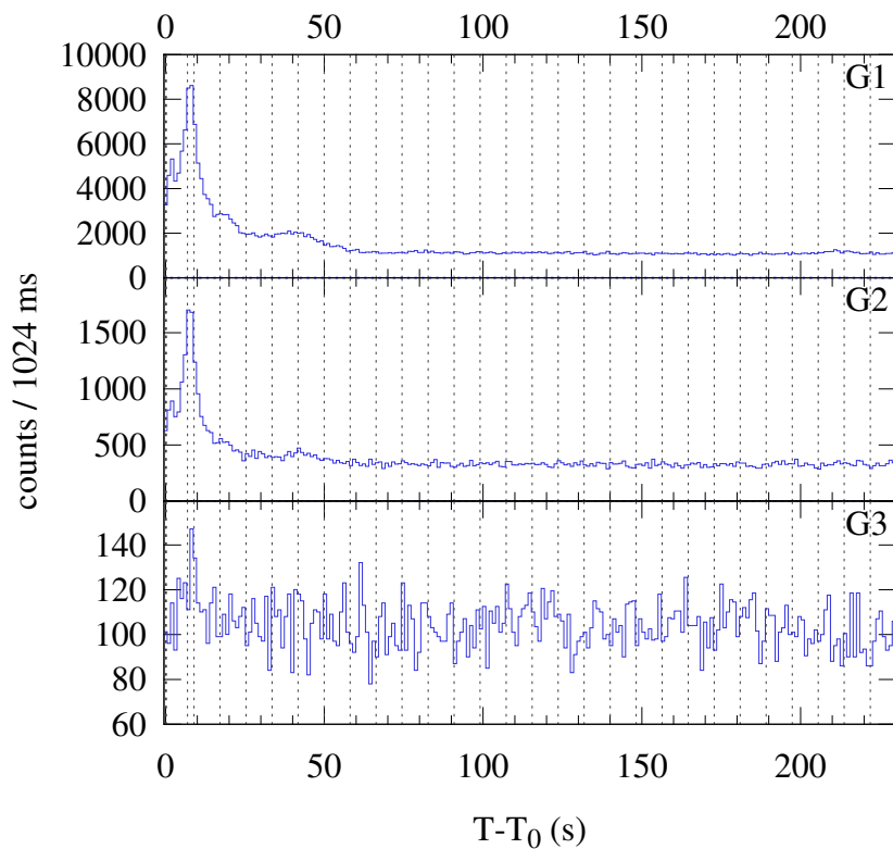
Konus-WIND S2 SOL2024-12-12T17:39 (M2.2) T_0 = 63594.271 s UT (17:39:54.271)
