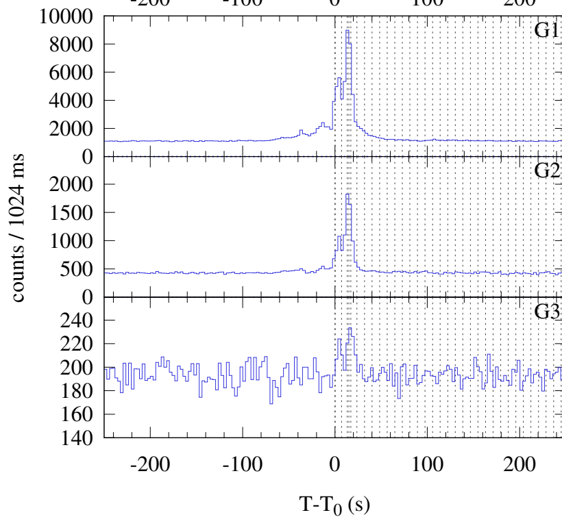
Konus-WIND S2 SOL2024-12-21T00:37 (M1.9) T_0 = 2259.56 s UT (00:37:39.56)
