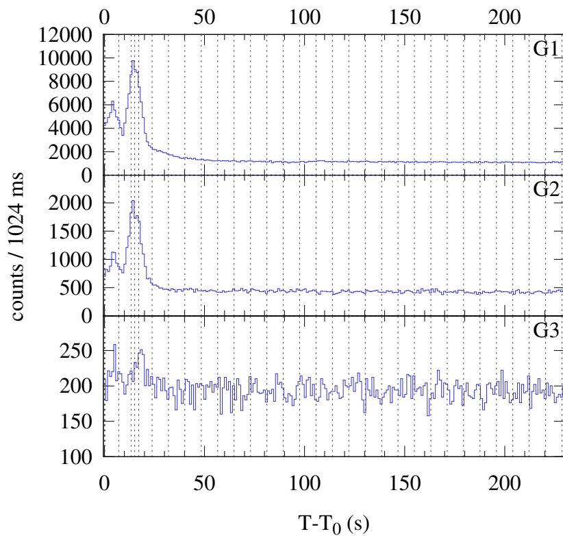
Konus-WIND S2 SOL2024-12-21T00:37 (M1.9) T_0 = 2259.56 s UT (00:37:39.56)
