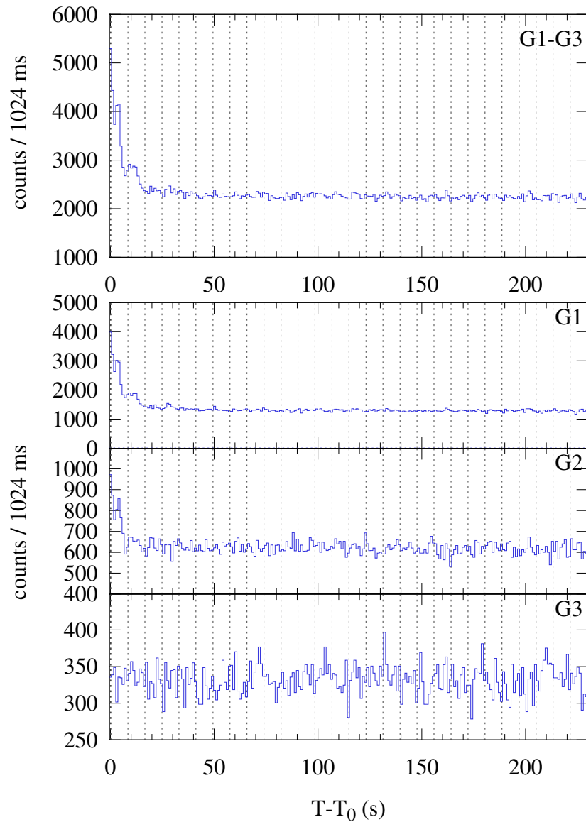
Konus-WIND S2 SOL2024-12-22T04:09 (M1.0) T_0 = 14981.462 s UT (04:09:41.462)
