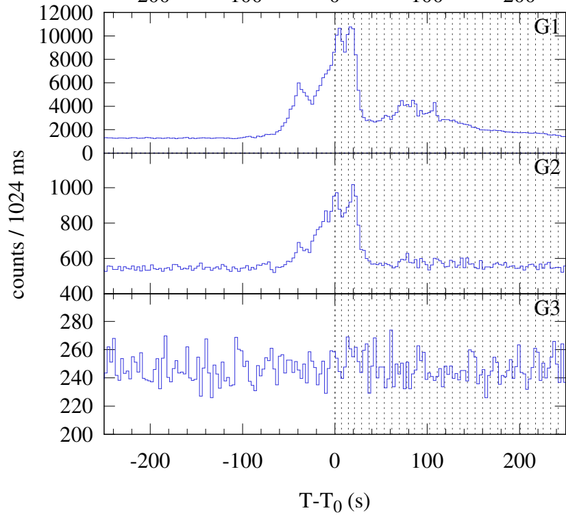
Konus-WIND S2 SOL2024-12-23T11:09 (M8.9) T_0 = 40152.468 s UT (11:09:12.468)
