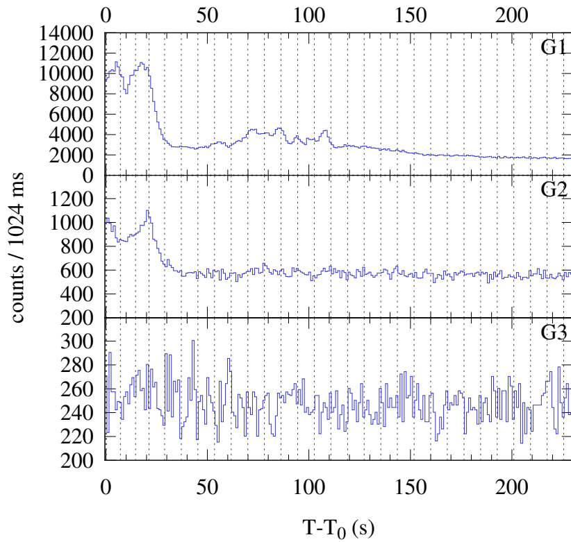
Konus-WIND S2 SOL2024-12-23T11:09 (M8.9) T_0 = 40152.468 s UT (11:09:12.468)
