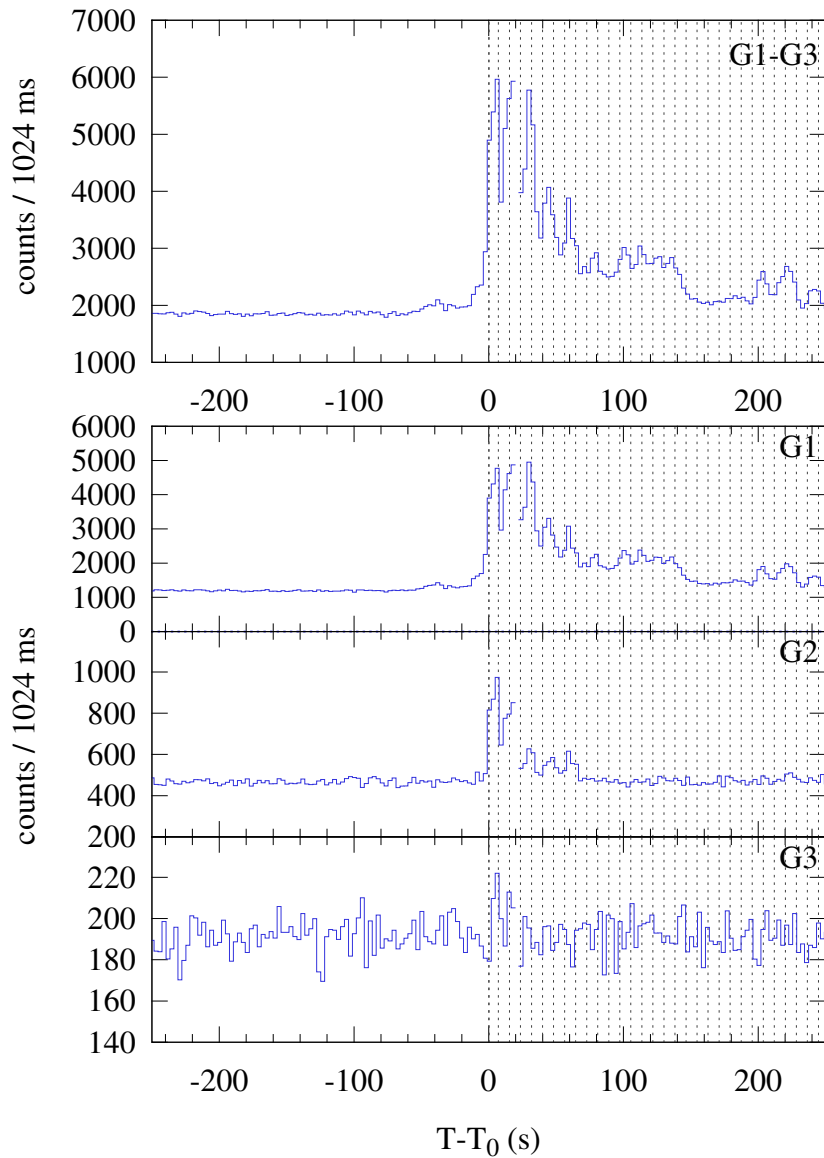
Konus-WIND S2 SOL2024-12-24T08:38 (M4.1) T 0 = 31098.846 s UT (08:38:18.846)
