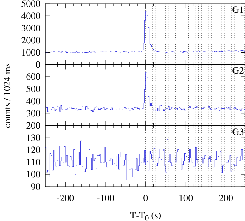
Konus-WIND S2 SOL2024-12-29T04:19 (M2.0) T 0 = 15579.55 s UT (04:19:39.55)
