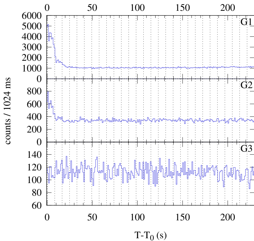
Konus-WIND S2 SOL2024-12-29T04:19 (M2.0) T 0 = 15579.55 s UT (04:19:39.55)
