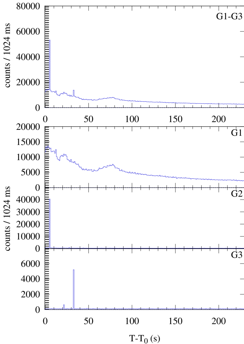
Konus-WIND S2 SOL2024-12-29T15:06 (M7.1) T_0 = 54392.858 s UT (15:06:32.858)
