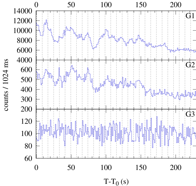
Konus-WIND S2 SOL2025-01-04T12:42 (X1.8) T_0 = 45765.821 s UT (12:42:45.821)
