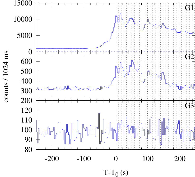
Konus-WIND S2 SOL2025-01-04T12:42 (X1.8) T_0 = 45765.821 s UT (12:42:45.821)
