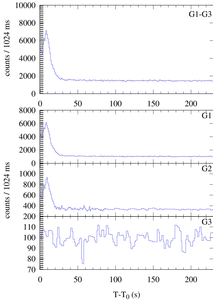
Konus-WIND S2 SOL2025-02-05T18:27 (C4.4) T 0 = 66436.582 s UT (18:27:16.582)
