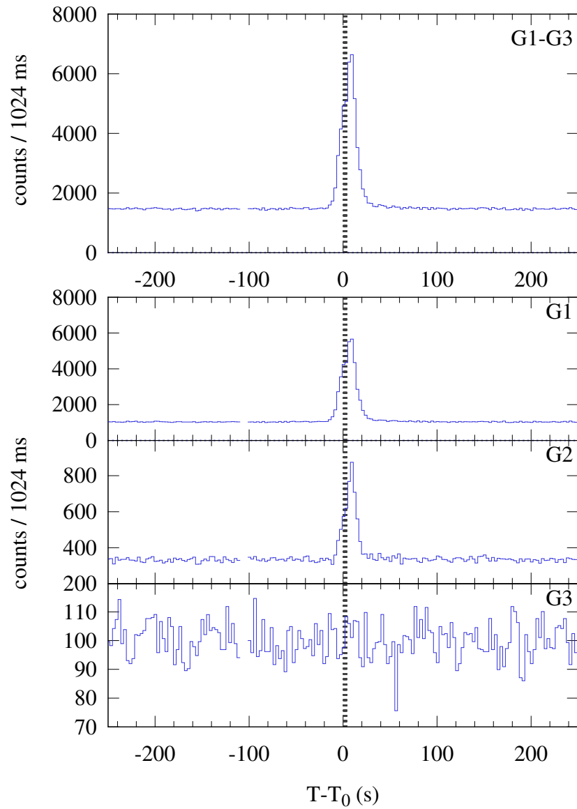
Konus-WIND S2 SOL2025-02-05T18:27 (C4.4) T 0 = 66436.582 s UT (18:27:16.582)
