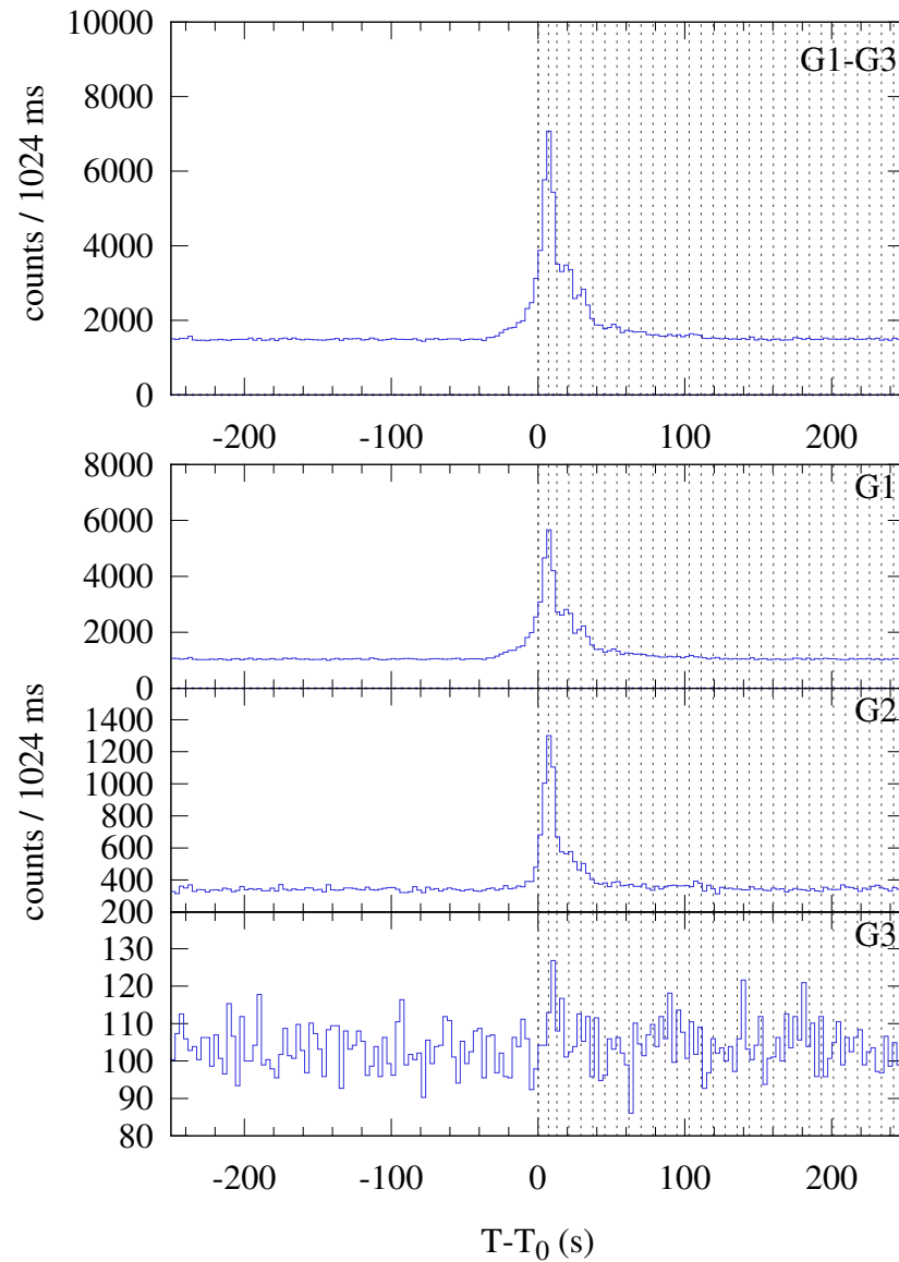
Konus-WIND S2 SOL2025-03-11T13:03 (M1.1) T_0 = 47018.228 s UT (13:03:38.228)
